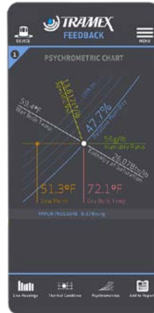
Psychrometric Chart
